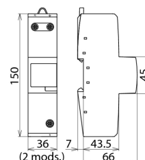
Dimension drawing DGPM 440
