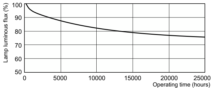
Lumen Maintenance Diagram - MASTER TL-D Food 30W/79 SLV/25
