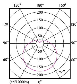
Light Distribution Diagram - PILA LED 100W A60 E27 CW FR ND 1CT/6 G3
