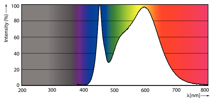
Spectral Power Distribution Colour - PILA LED 100W A60 E27 CW FR ND 1CT/6 G3
